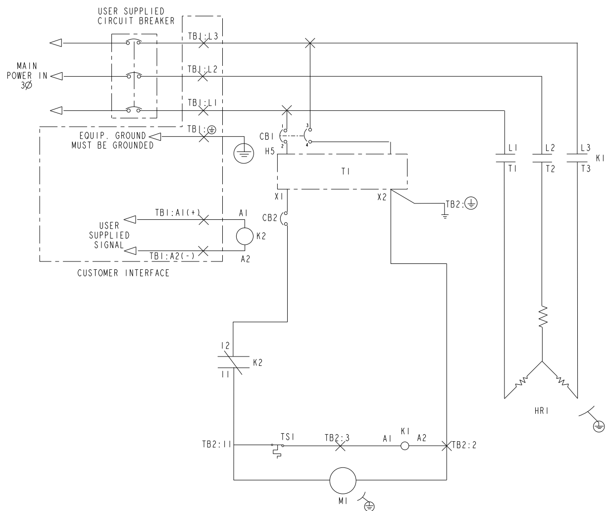
ELECTRICAL WIRING SCHEMATIC
