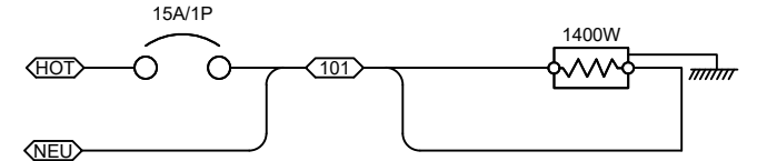
D Alternator Heater 120VAC
