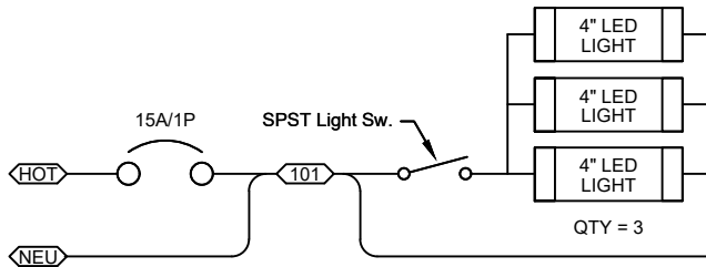
A Enclosure Interior Switched Fluorescent Lighting Detail (AC)
