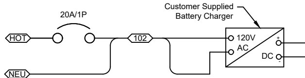
F Battery Charger mounting and feeder
