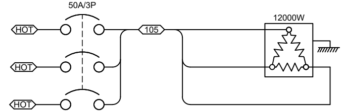
E Jacket Water Heater 208VAC
