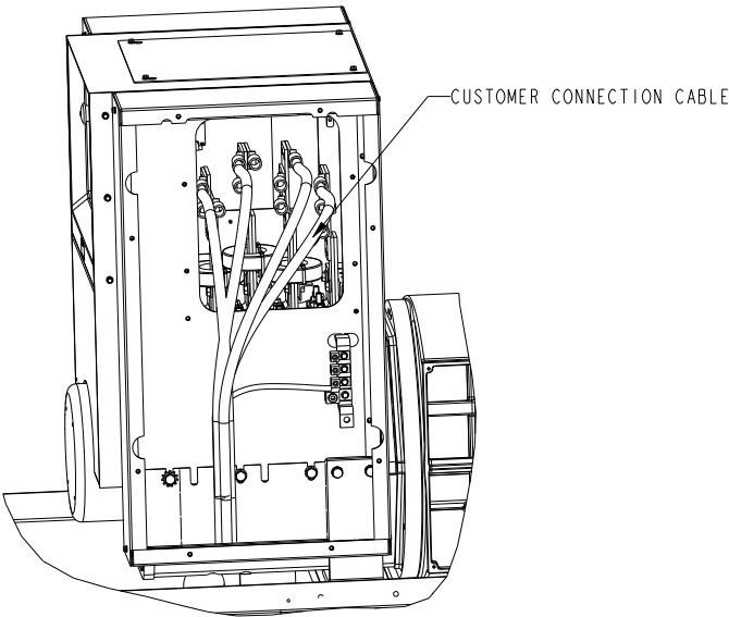
ONE CONDUIT WIRED FOR REFERENCE ONLY
