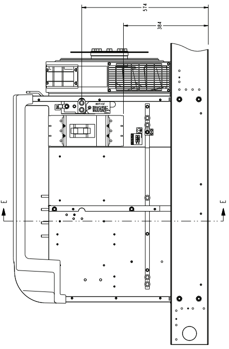
"L" FRAME SHOWN (400 - 600 amp)
